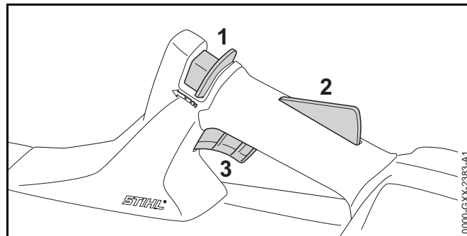
Retaining Latch (1), Ergo-Lever (2) and Trigger Switch (3)
